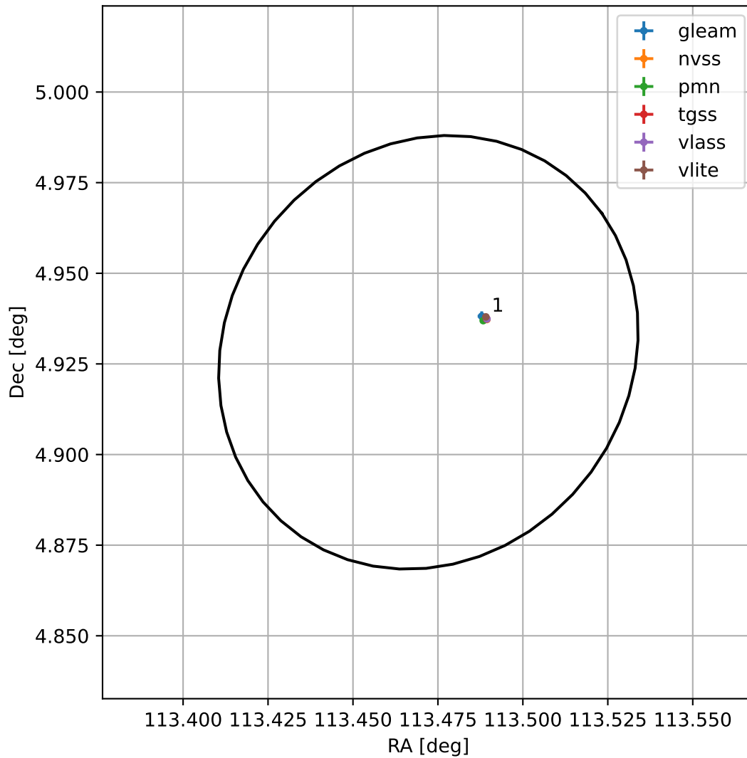
4FGL J0733.8+0455
