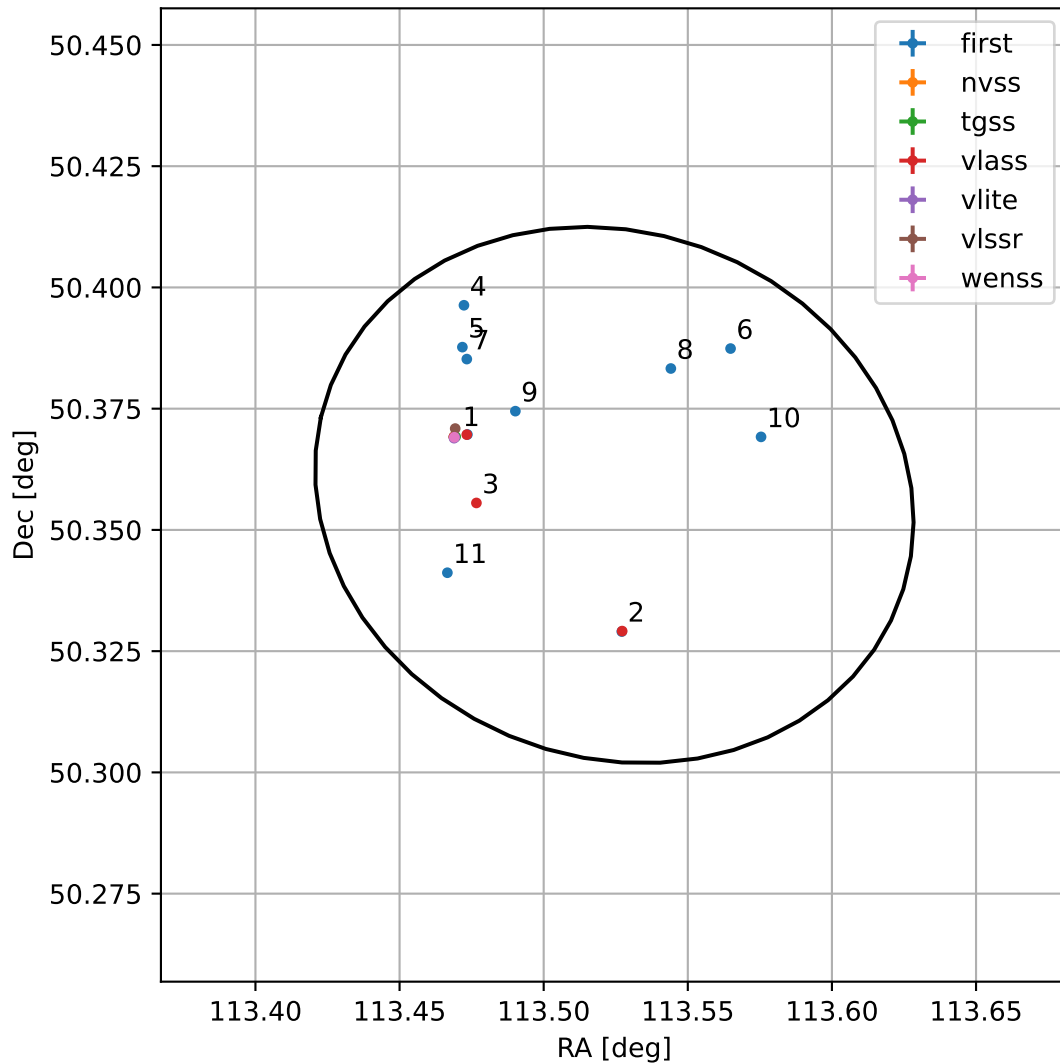
4FGL J0734.0+5021
