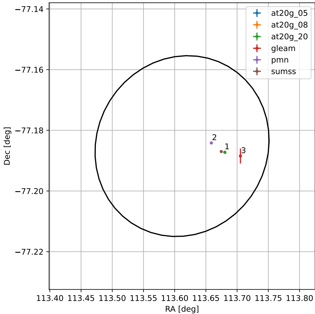
4FGL J0734.4-7711
