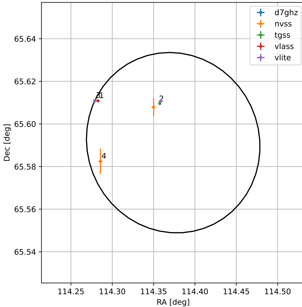
4FGL J0737.4+6535
