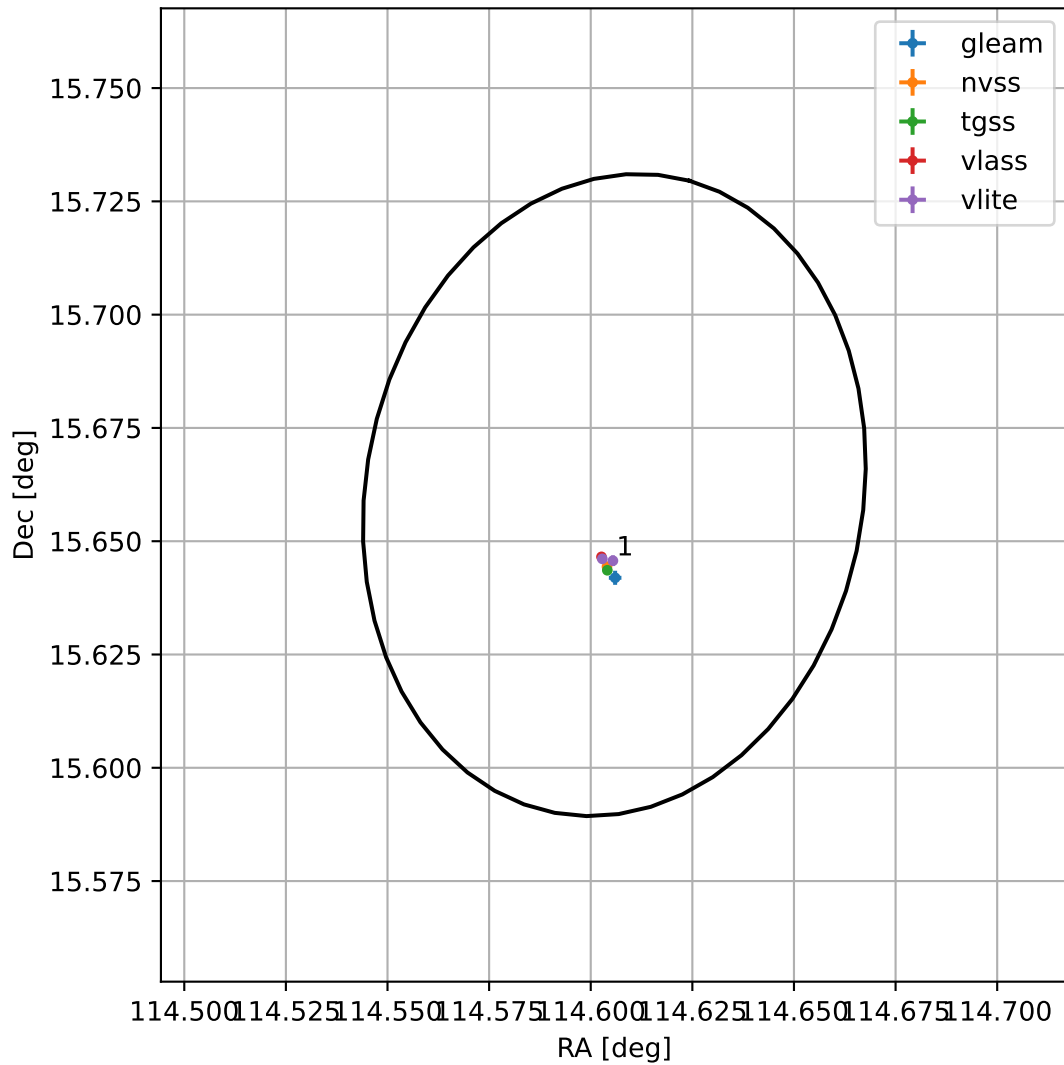
4FGL J0738.4+1539
