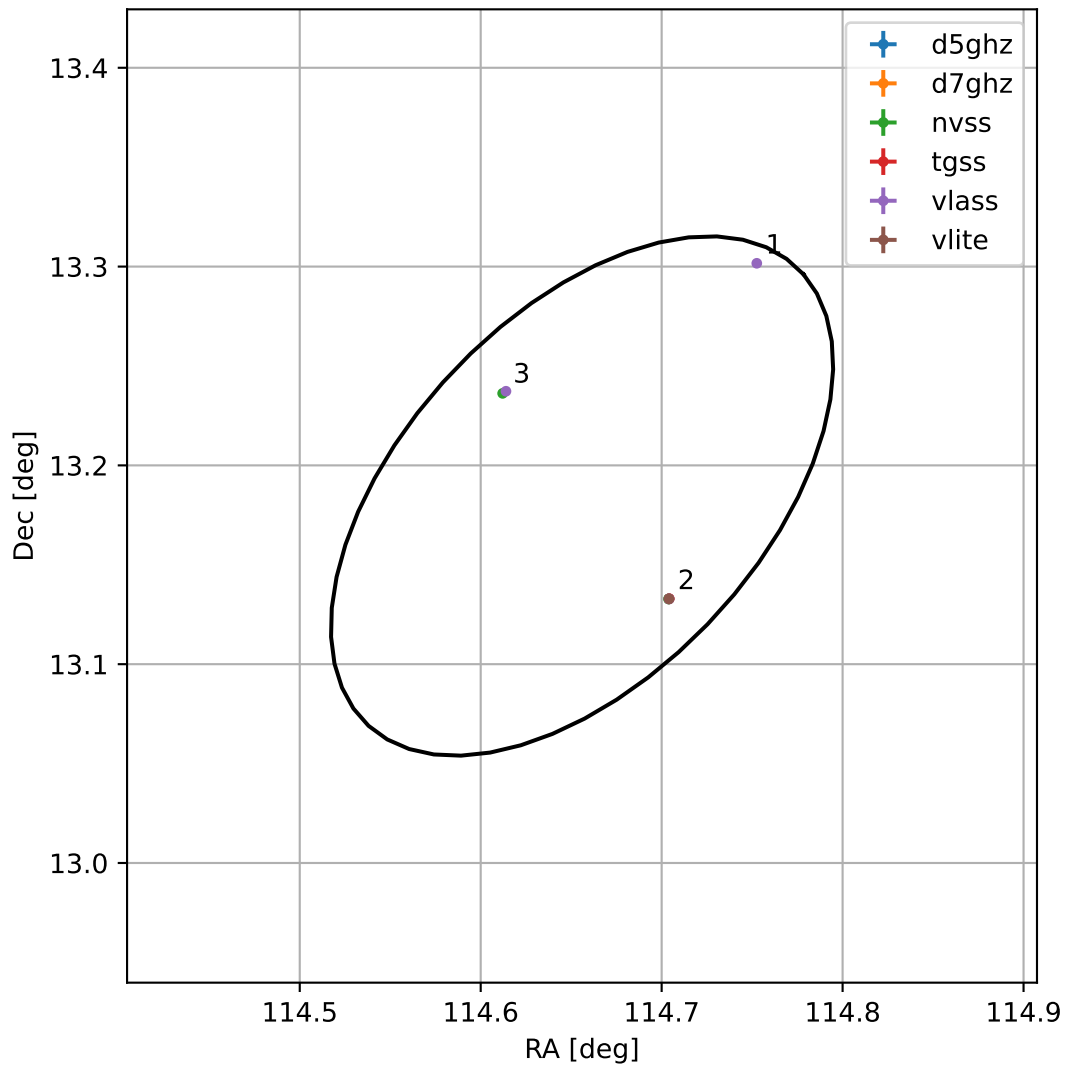
4FGL J0738.6+1311
