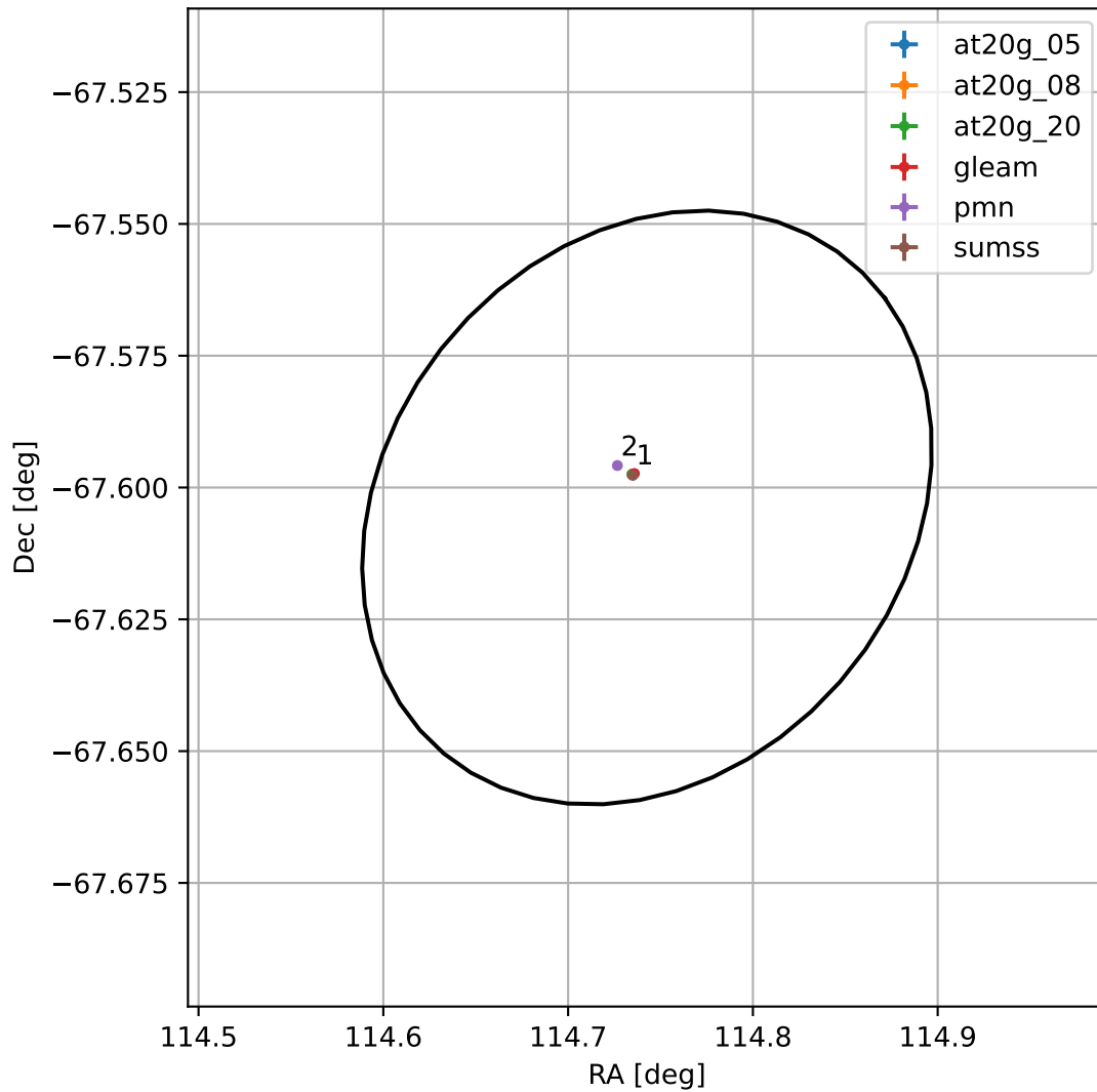
4FGL J0738.9-6736
