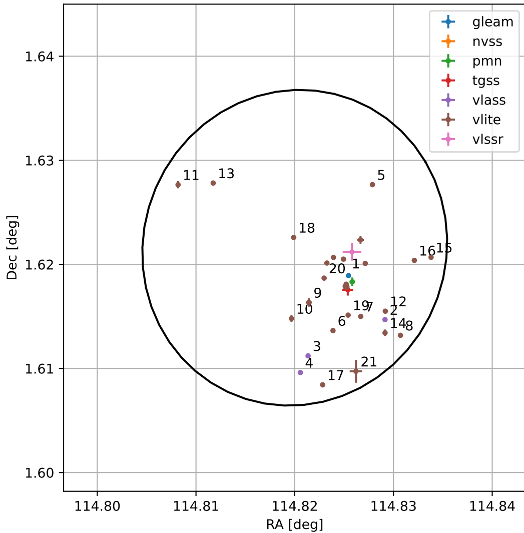
4FGL J0739.2+0137
