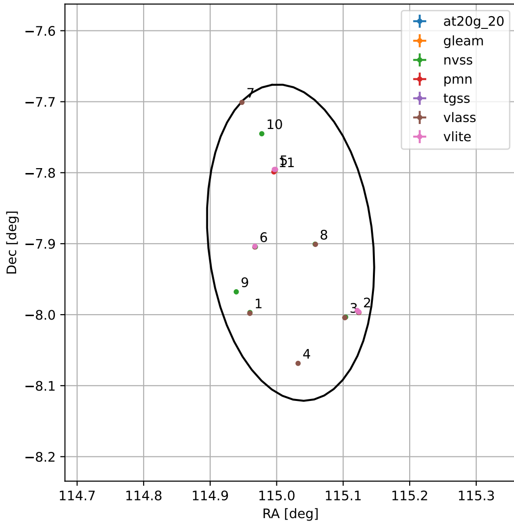
4FGL J0740.0-0753
