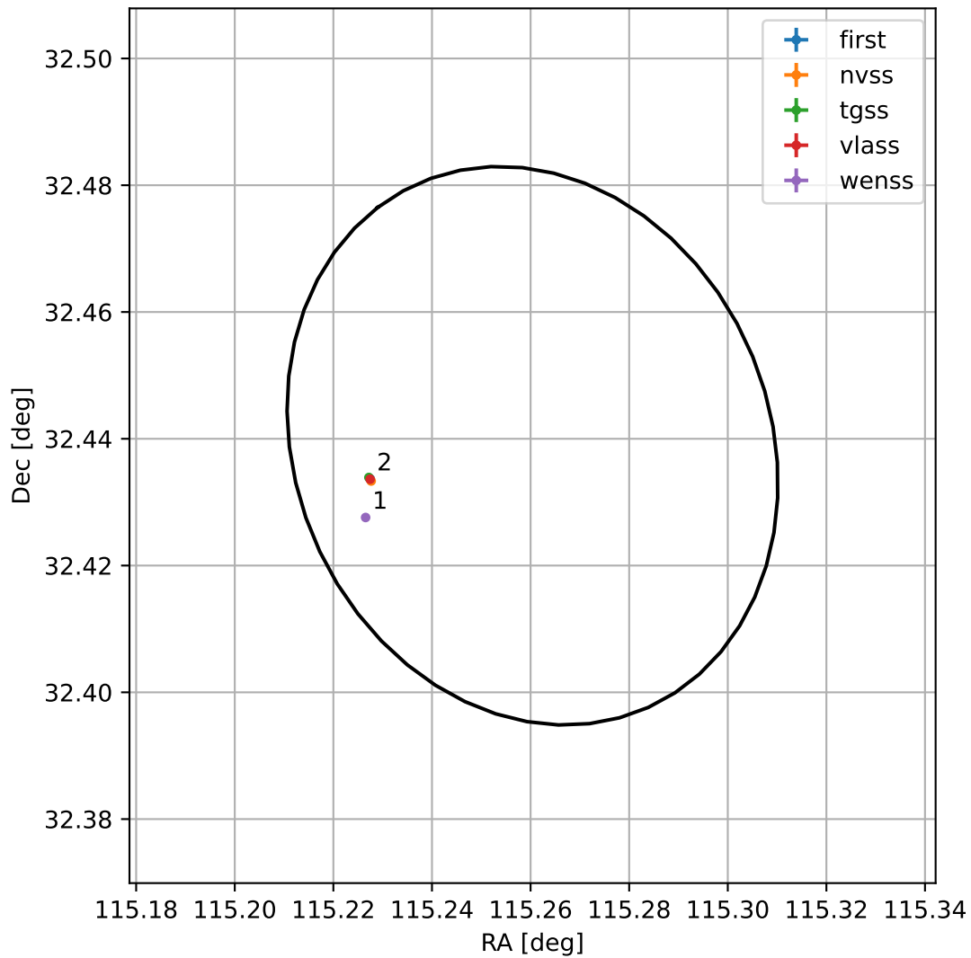
4FGL J0741.0+3226
