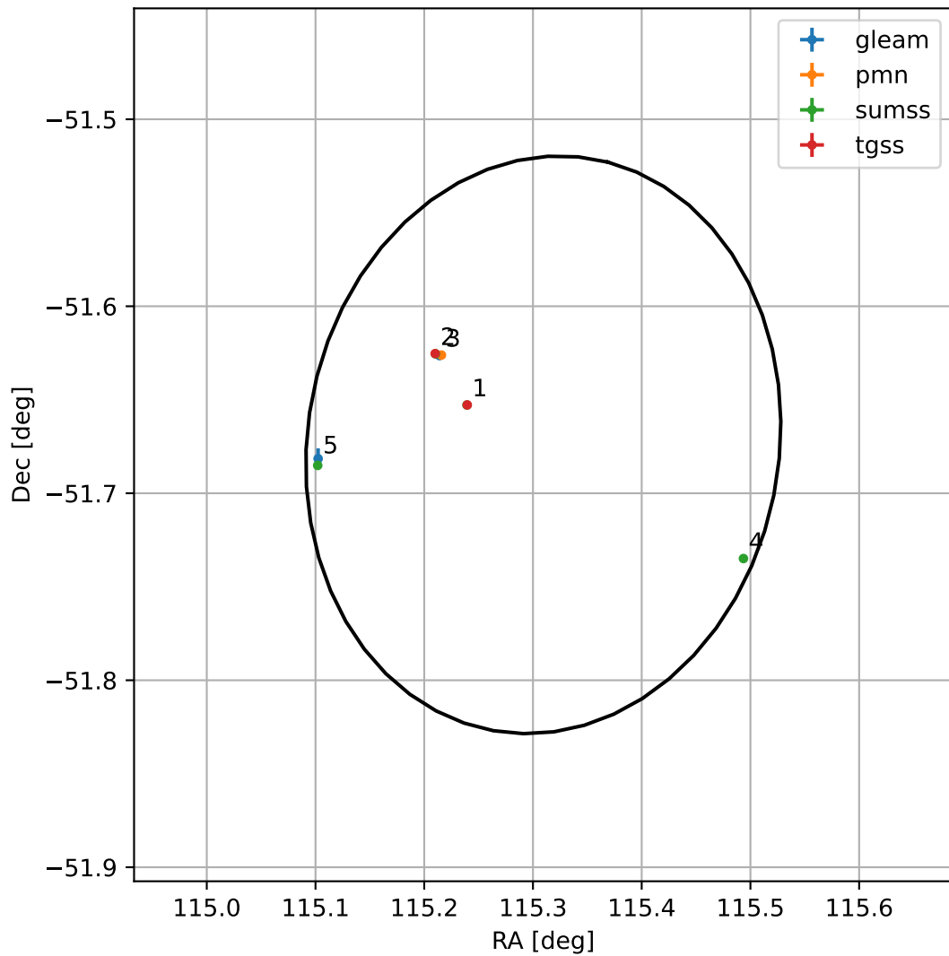
4FGL J0741.2-5140
