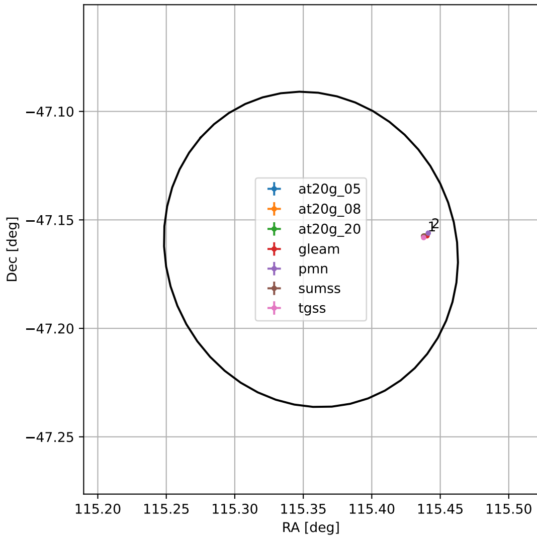
4FGL J0741.4-4709
