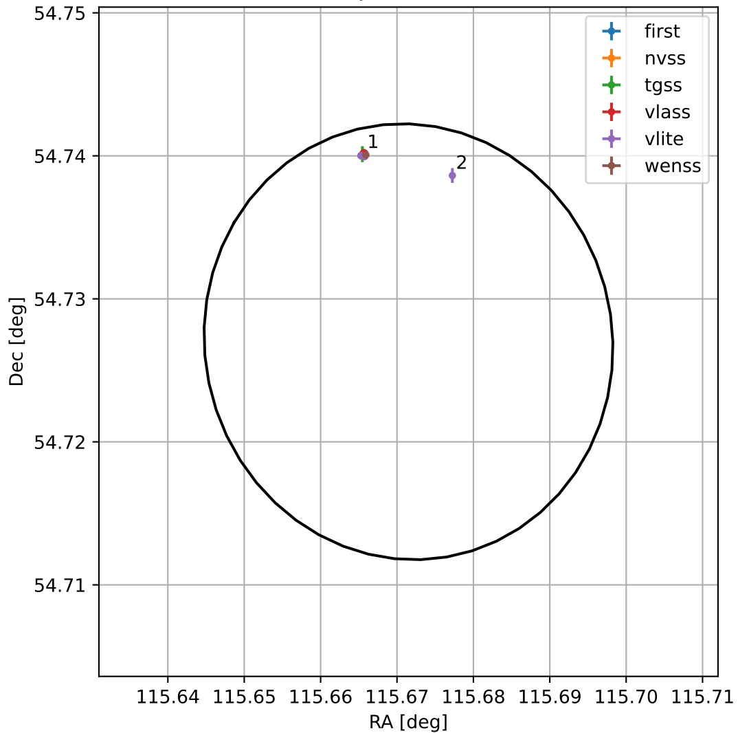
4FGL J0742.6+5443
