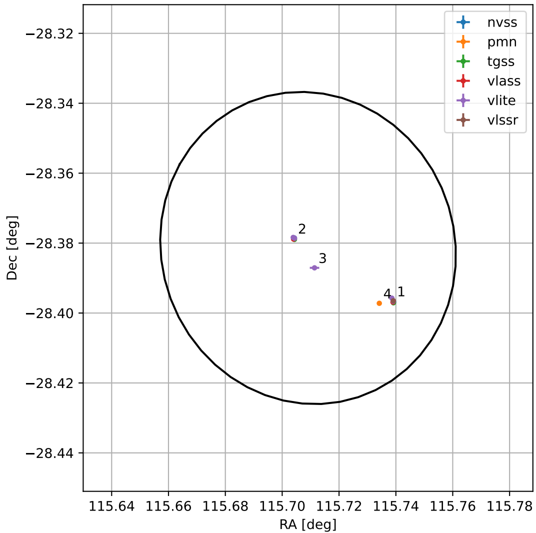
4FGL J0742.8-2822
