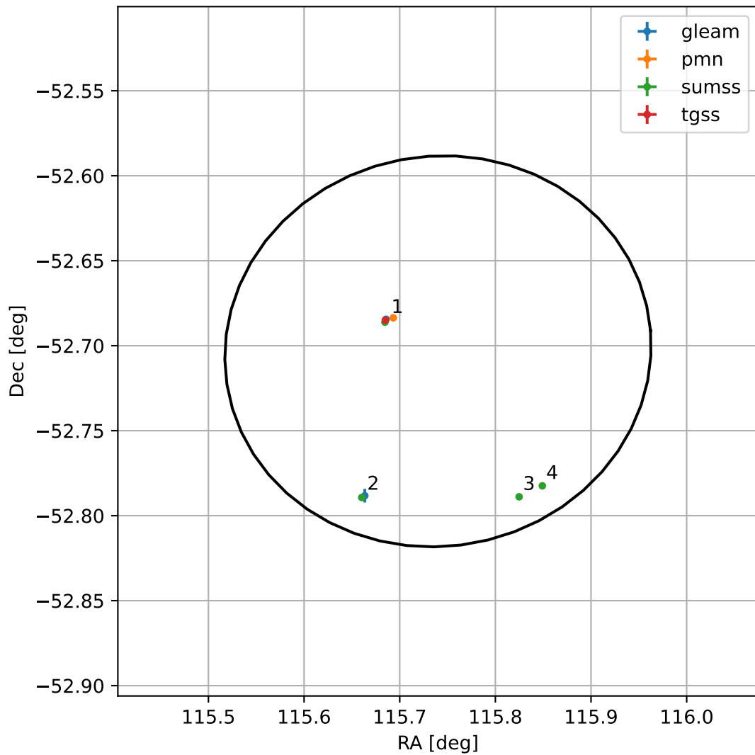
4FGL J0742.9-5242
