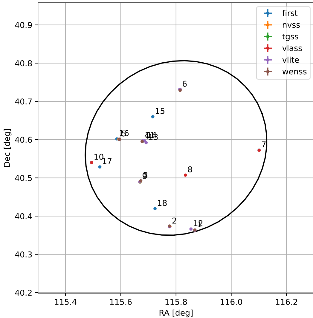
4FGL J0743.2+4034
