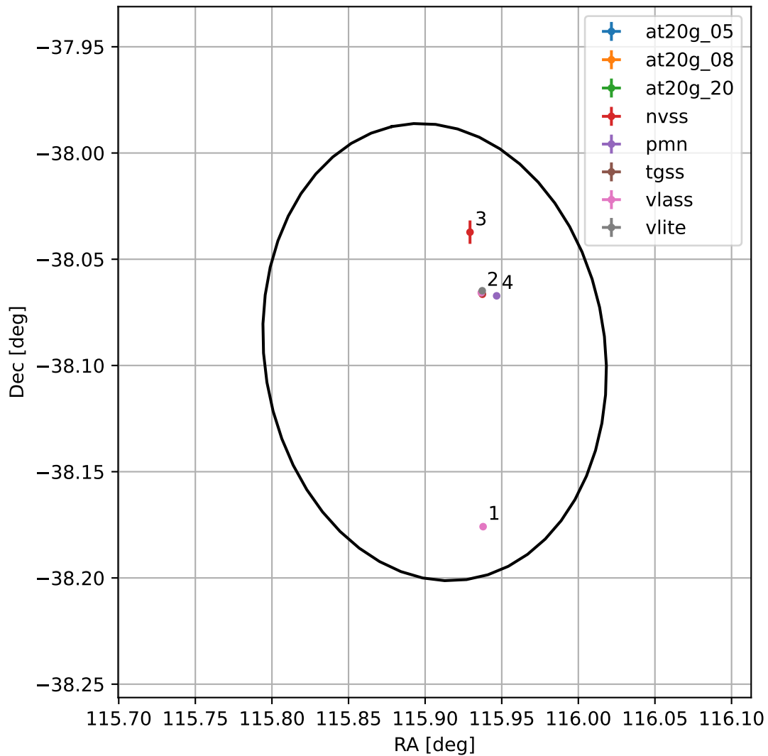
4FGL J0743.6-3805
