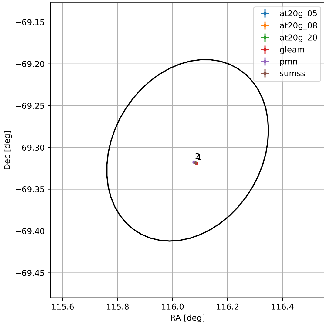
4FGL J0744.2-6918
