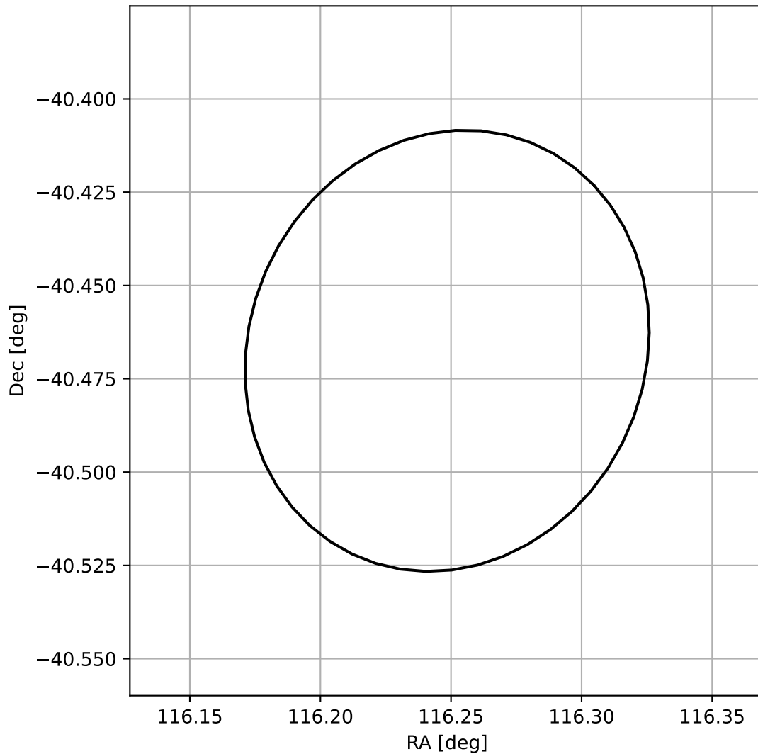
4FGL J0744.9-4028
