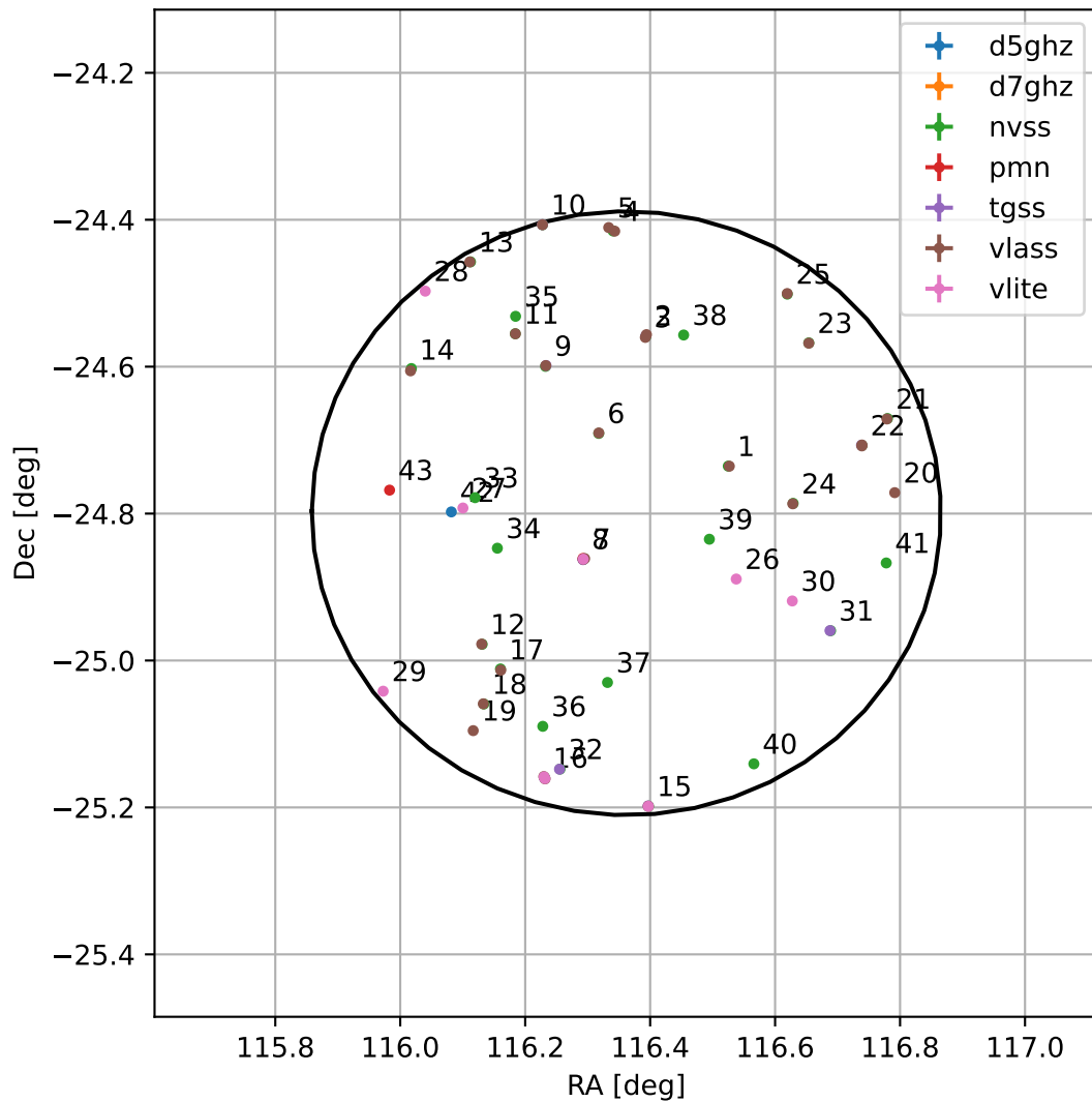
4FGL J0745.4-2447
