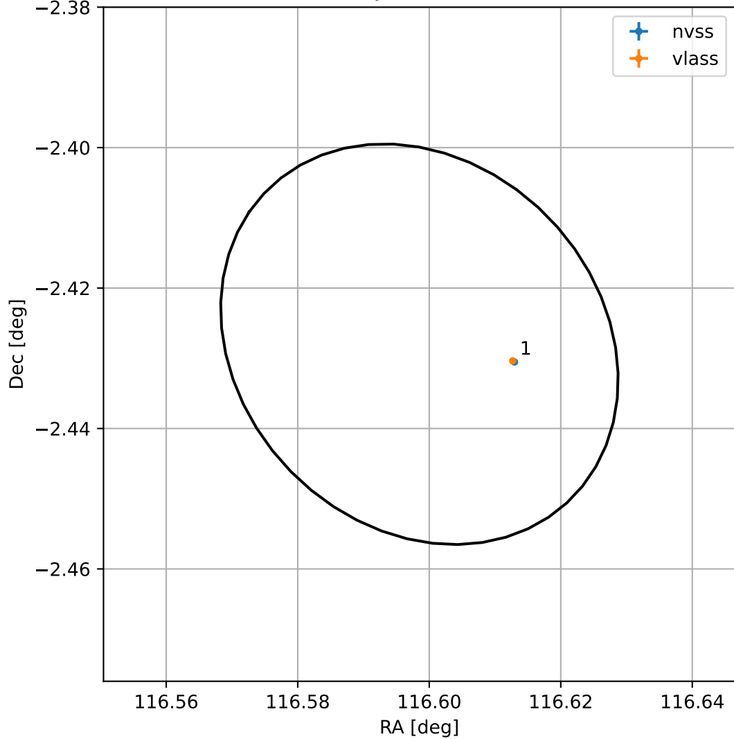
4FGL J0746.3-0225
