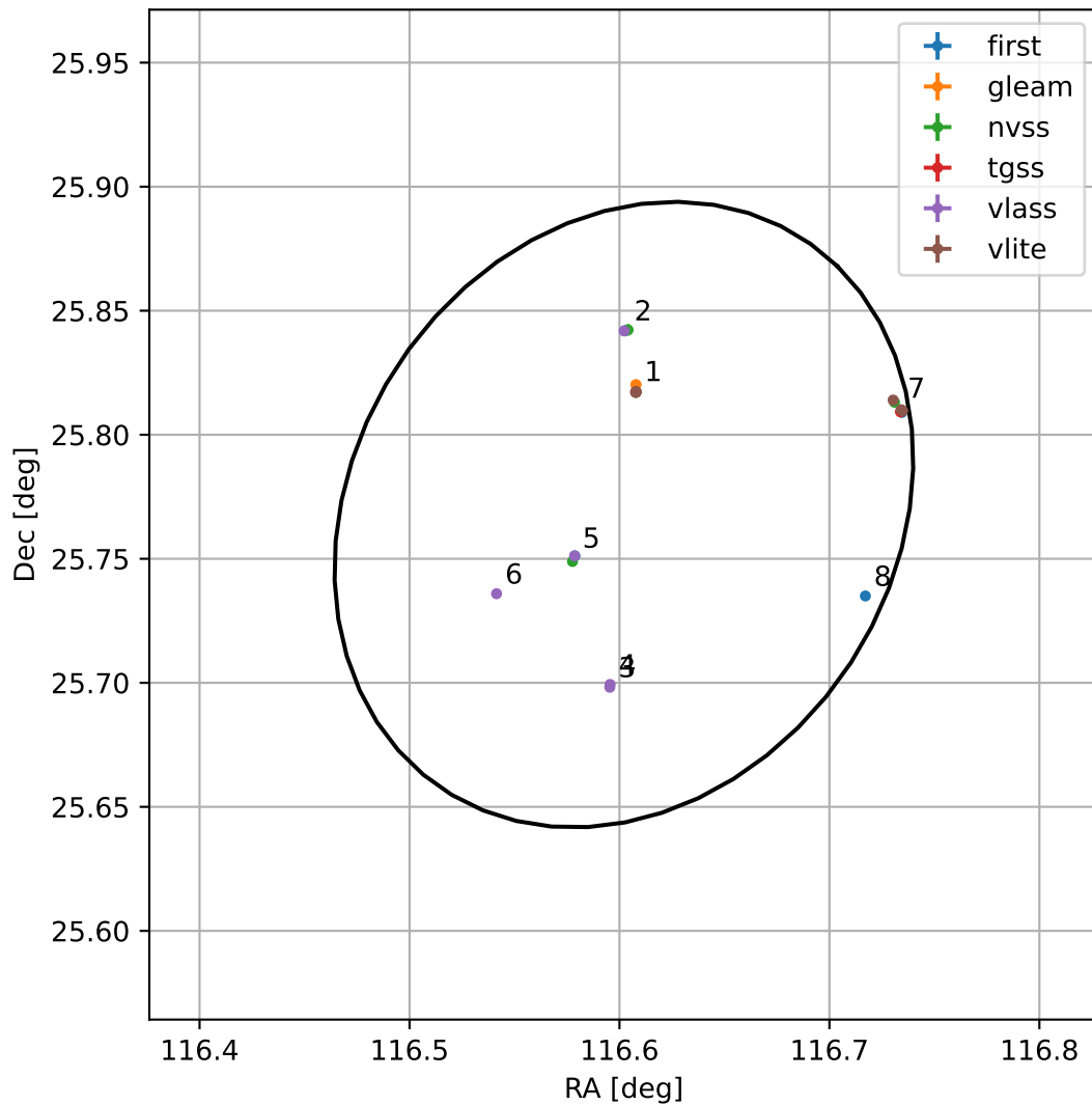
4FGL J0746.4+2546
