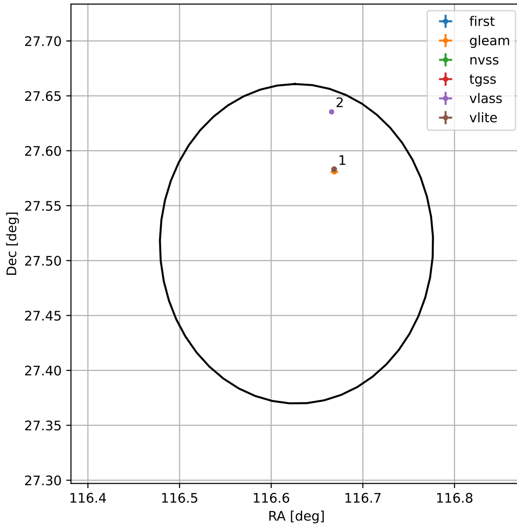
4FGL J0746.5+2730
