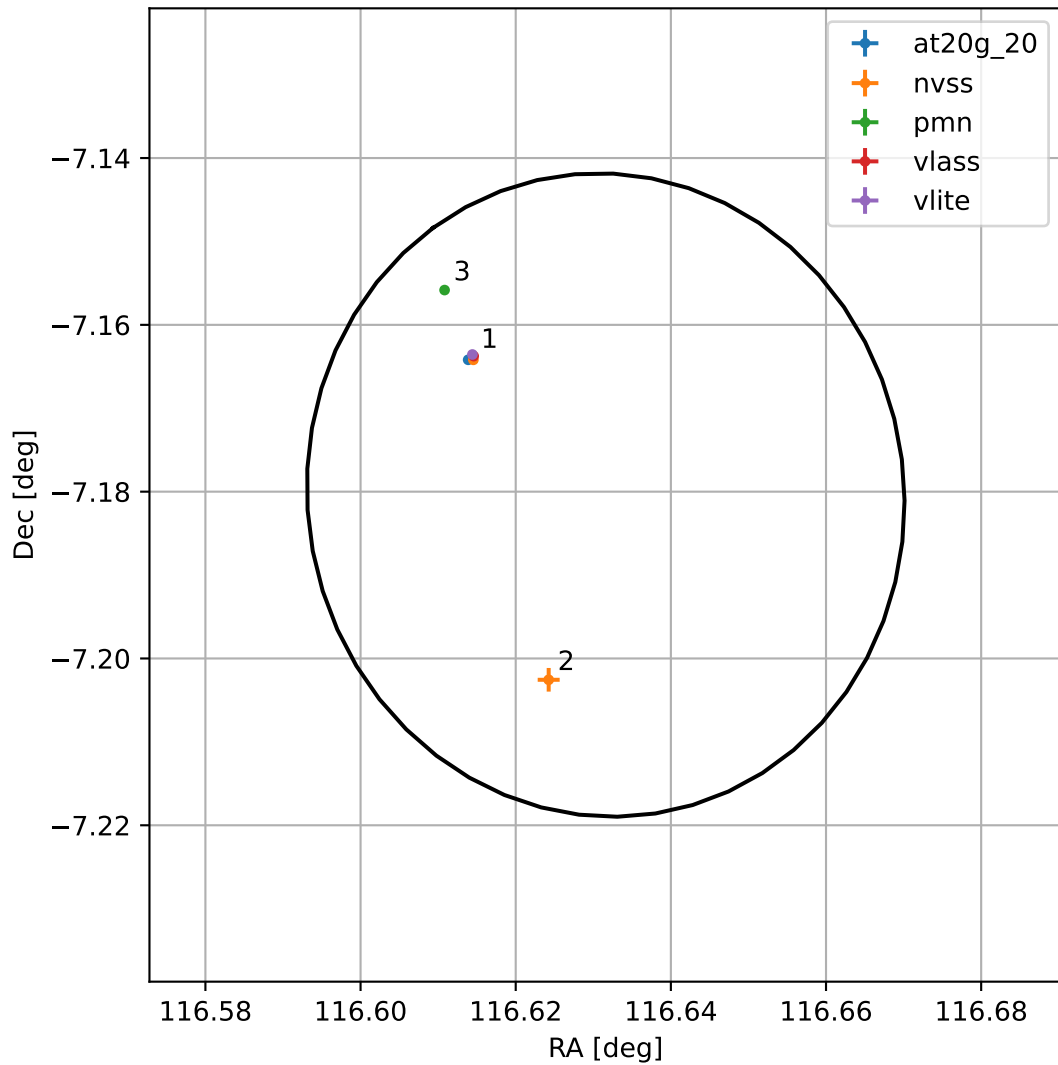
4FGL J0746.5-0710
