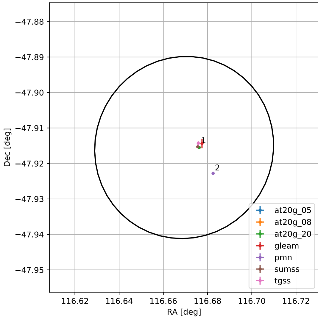
4FGL J0746.6-4754
