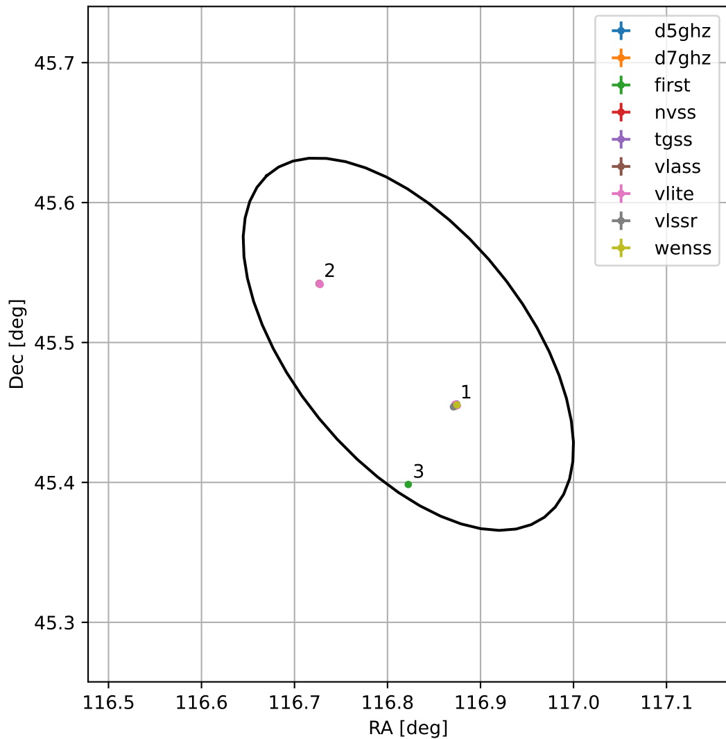
4FGL J0747.2+4529
