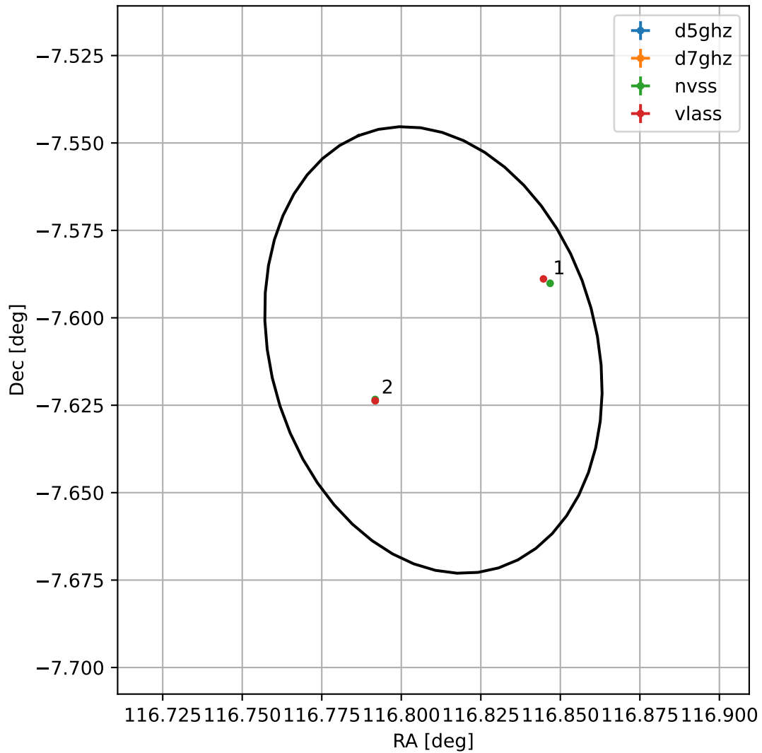
4FGL J0747.2-0736
