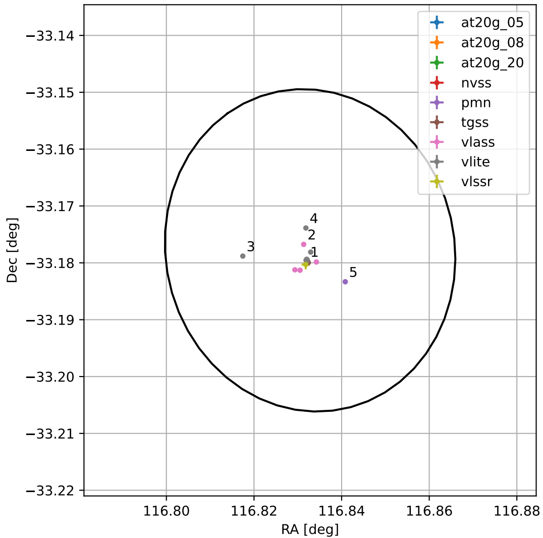
4FGL J0747.3-3310
