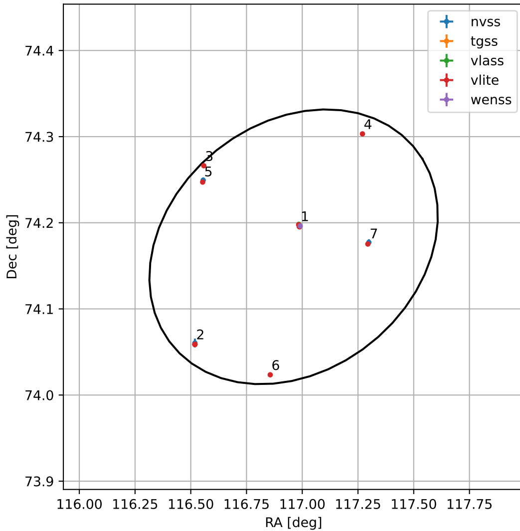
4FGL J0747.8+7410
