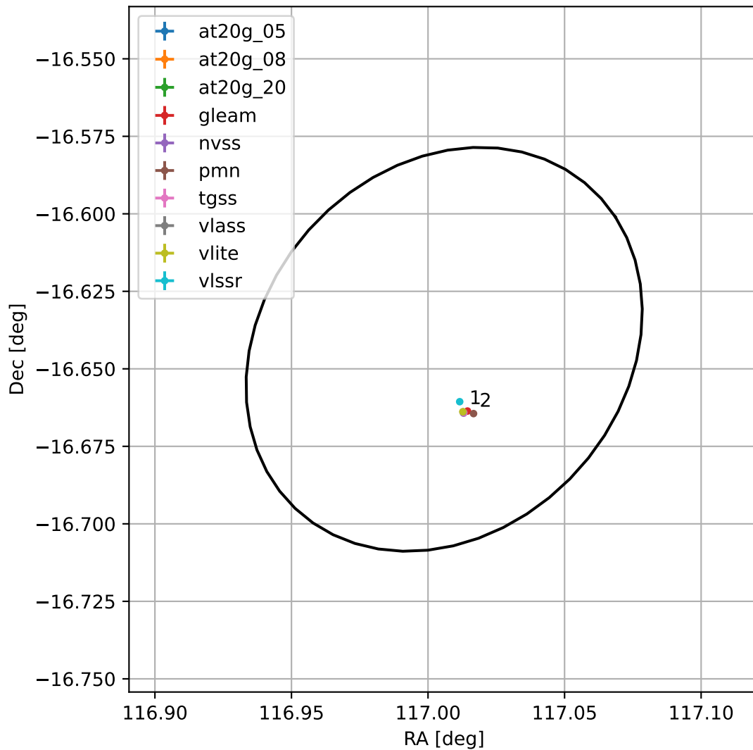
4FGL J0748.0-1638
