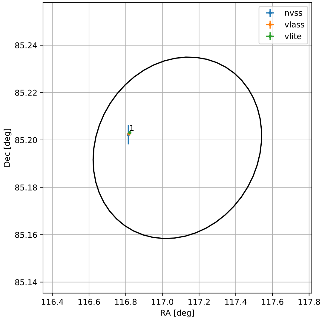
4FGL J0748.3+8511
