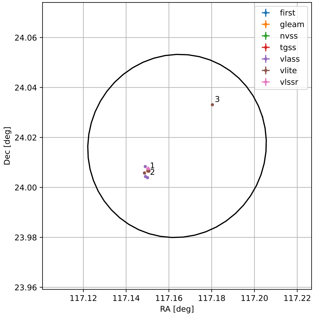
4FGL J0748.6+2400
