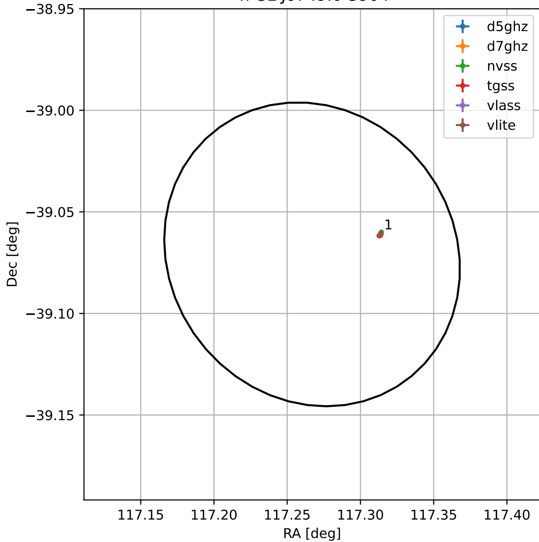
4FGL J0749.0-3904
