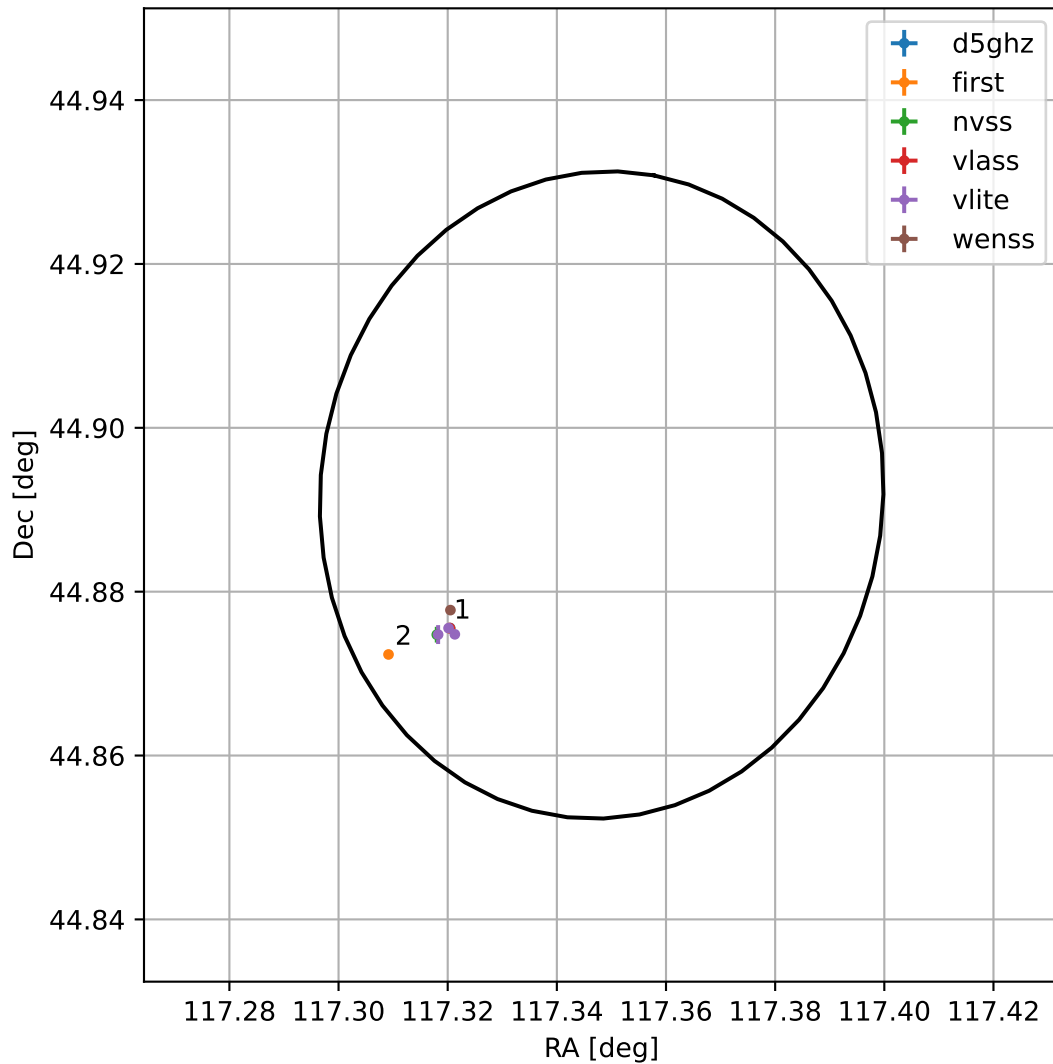
4FGL J0749.3+4453
