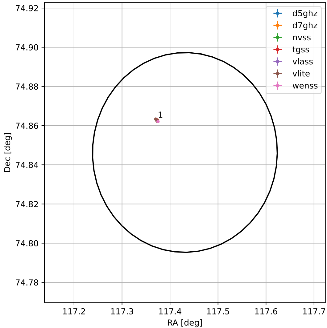
4FGL J0749.7+7450
