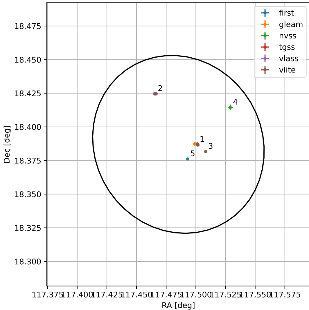
4FGL J0749.9+1823
