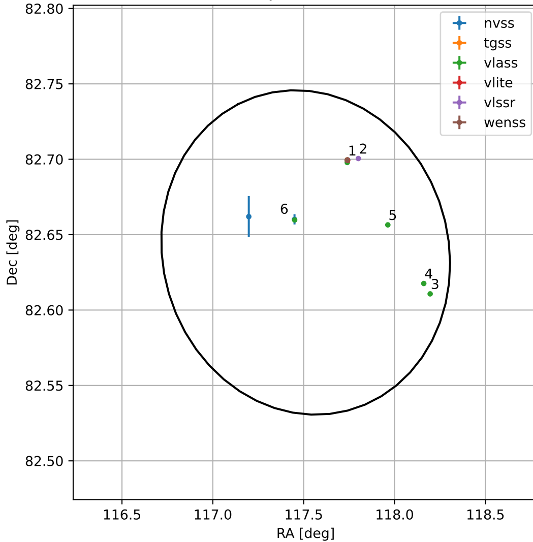
4FGL J0750.0+8238
