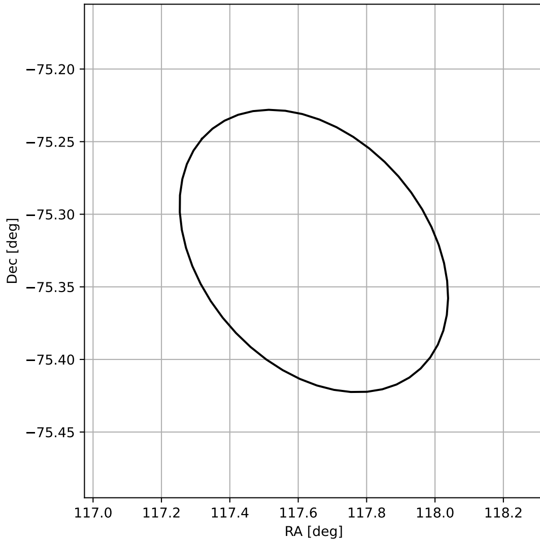
4FGL J0750.5-7519
