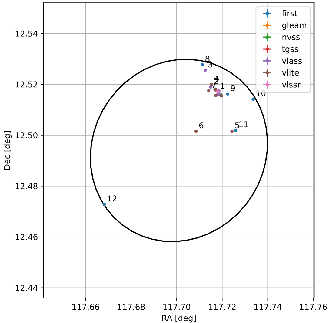
4FGL J0750.8+1229
