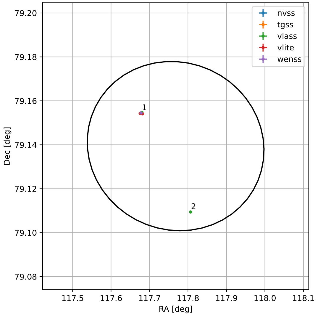
4FGL J0751.0+7908
