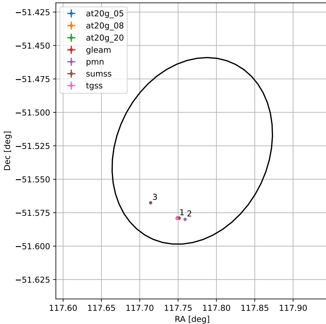
4FGL J0751.0-5131
