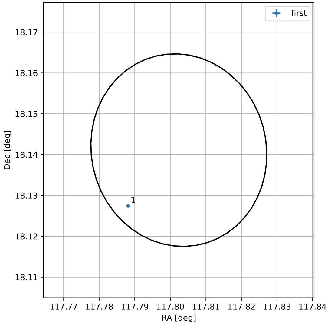
4FGL J0751.2+1808
