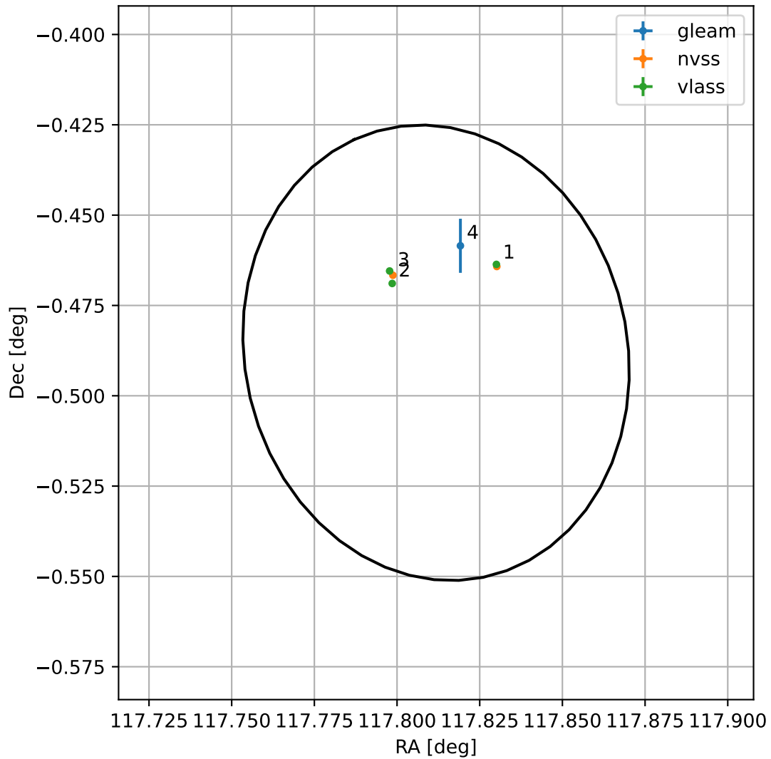
4FGL J0751.2-0029
