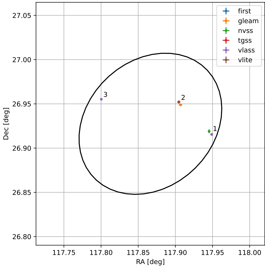
4FGL J0751.4+2655
