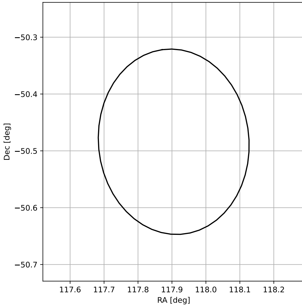
4FGL J0751.6-5029
