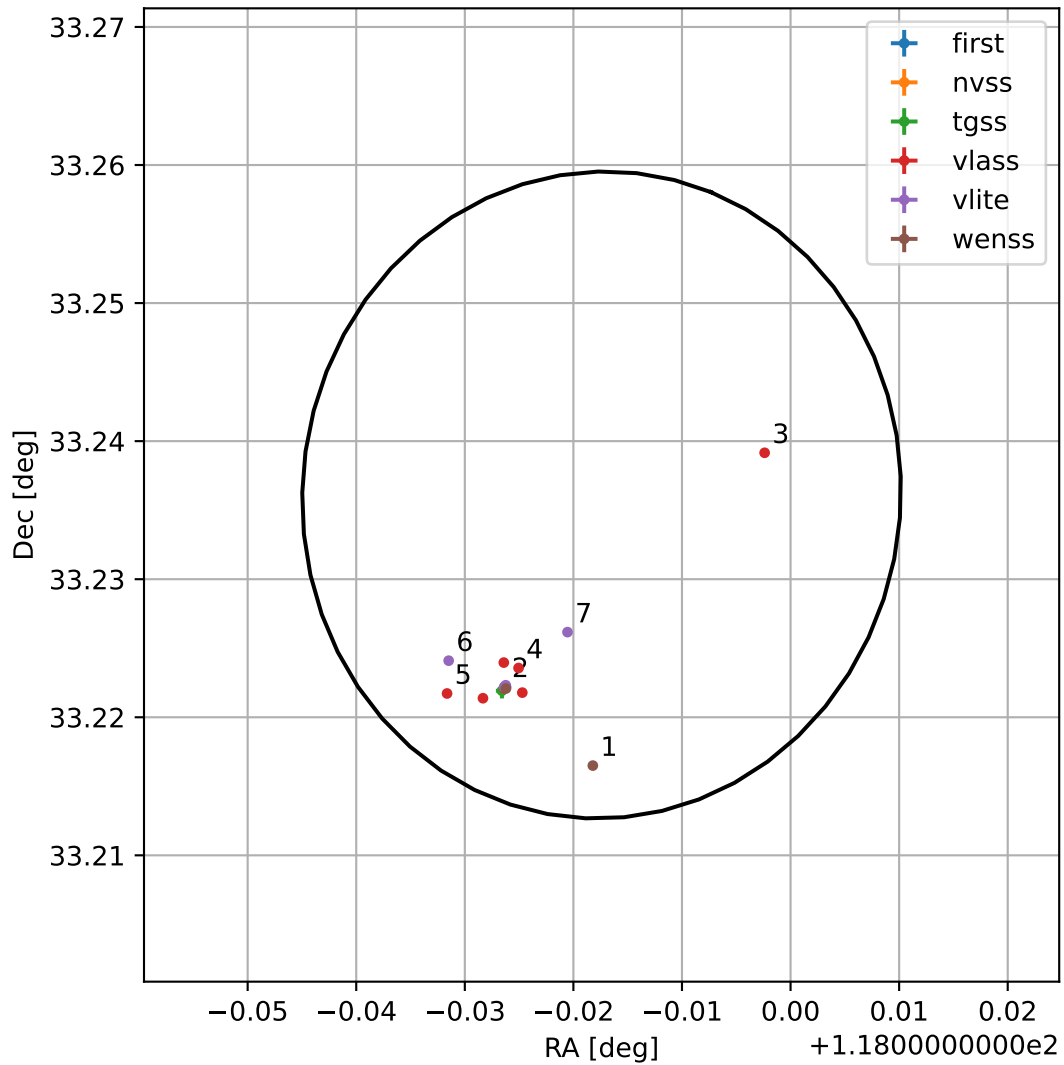
4FGL J0751.9+3314
