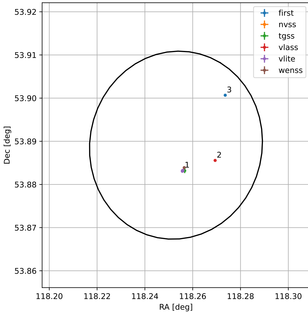
4FGL J0753.0+5353
