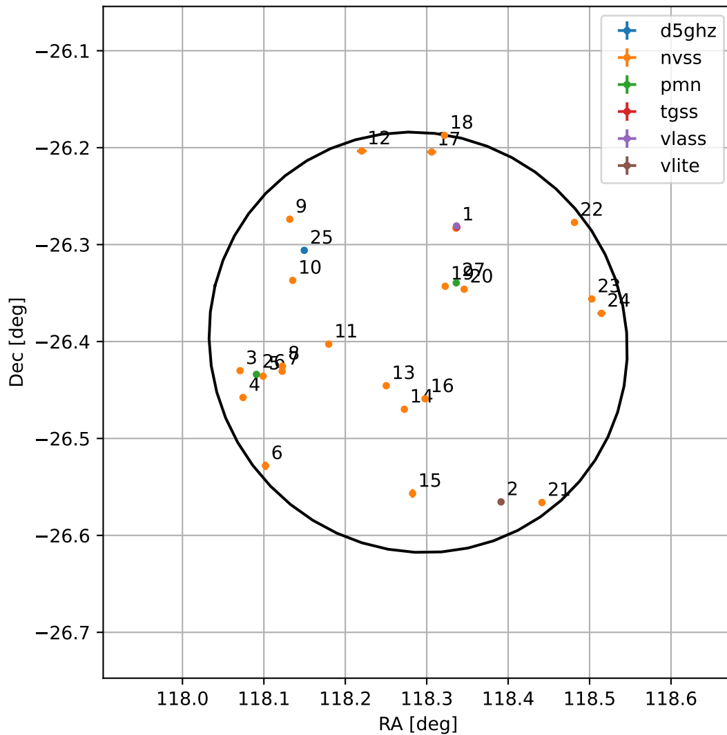
4FGL J0753.1-2624
