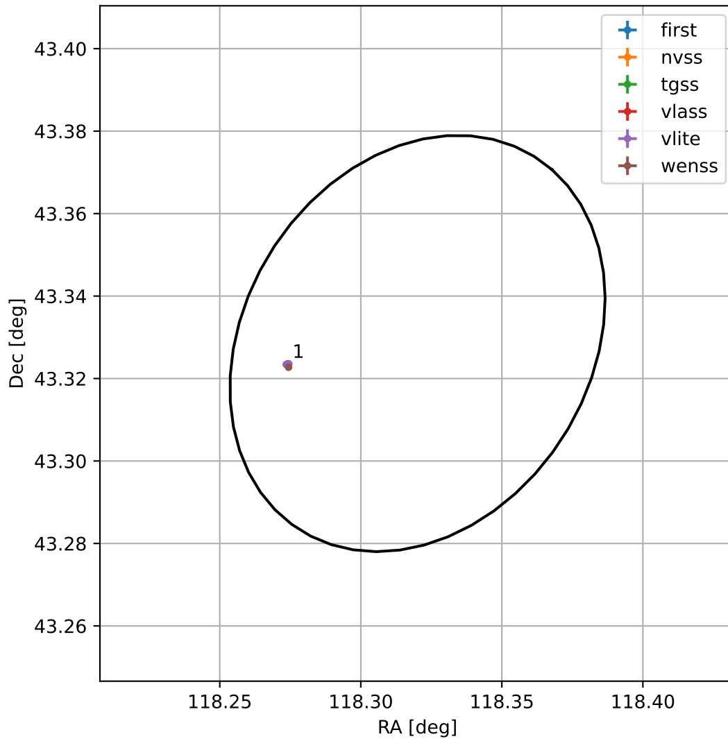
4FGL J0753.2+4319
