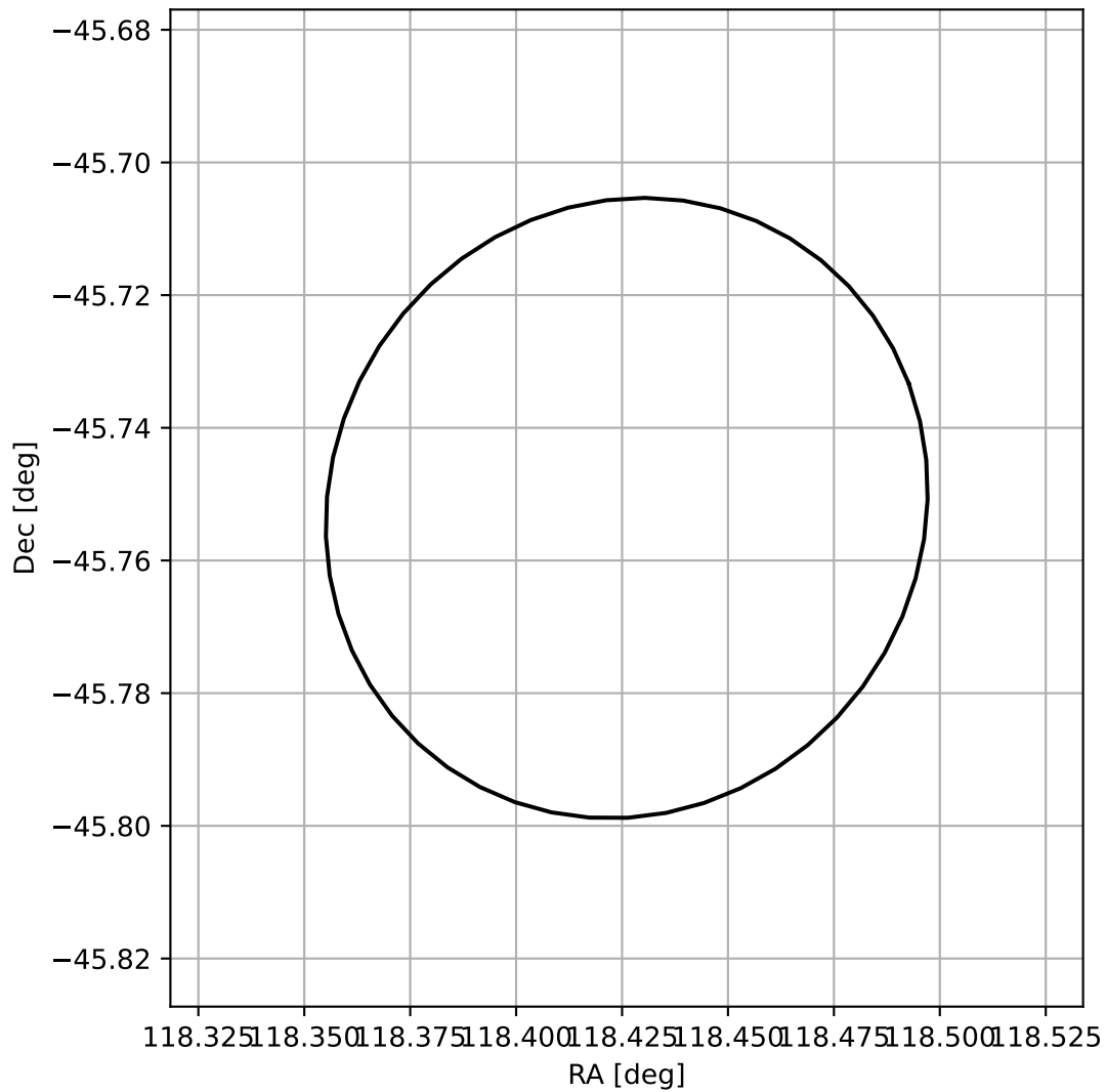
4FGL J0753.7-4545
